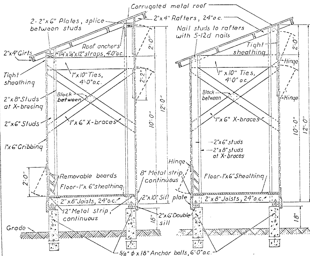
ALTERNATE FRAMING DETAIL SCALE 1/2" = 1'-0" THIS CONSTRUCTION REDUCES HEIGHT OF CRIB 6"
