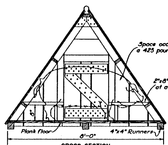
CROSS SECTION WITH FLOOR
