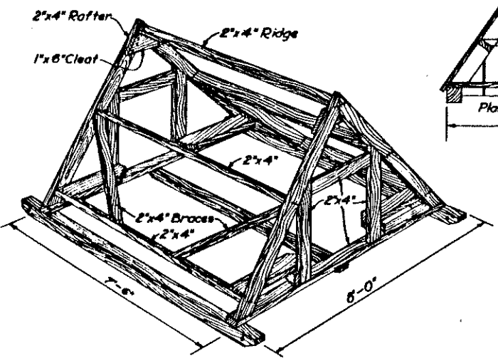
FRAMING PERSPECTIVE
