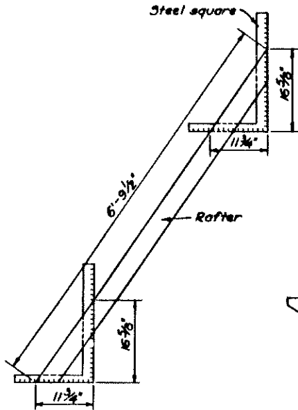
RAFTER CUTTING DETAIL
