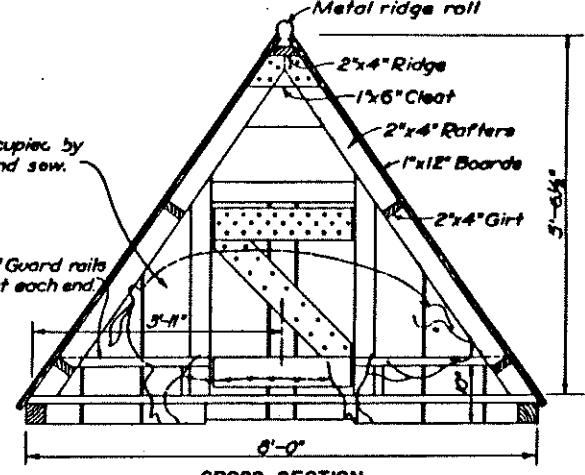
CROSS SECTION WITHOUT FLOOR
