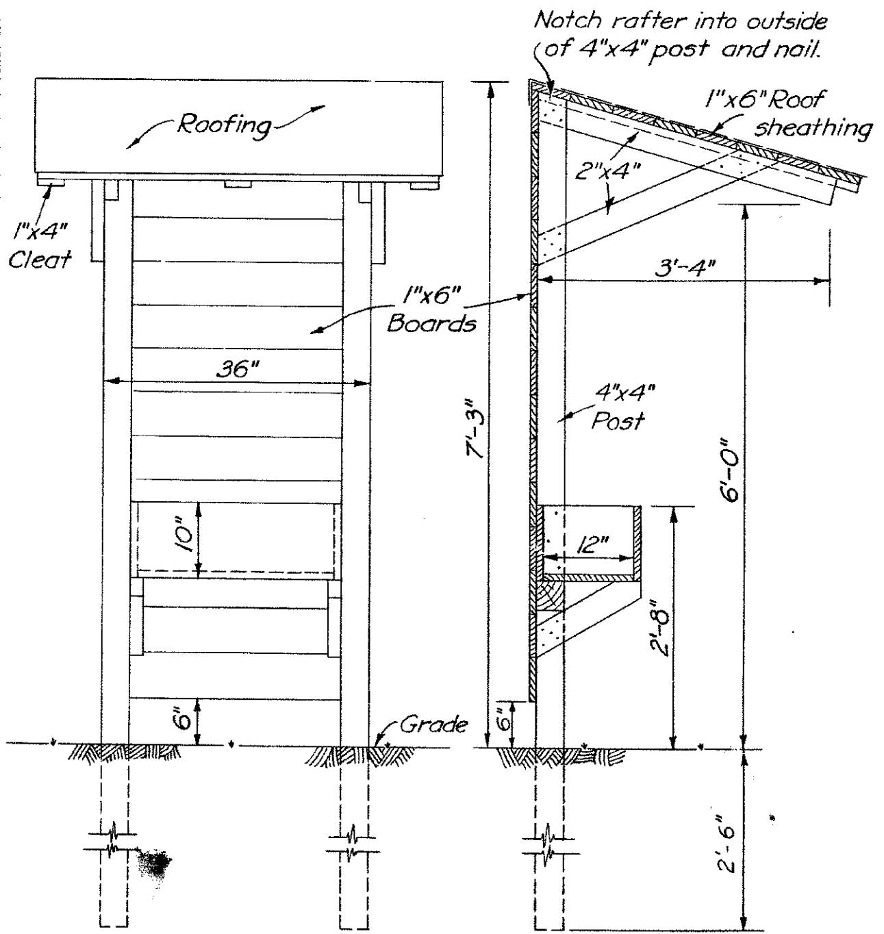
FRONT ELEVATION
