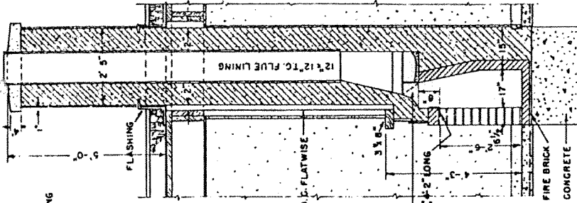
SECTION
