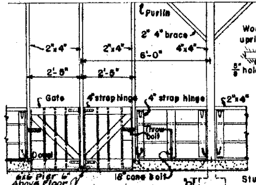
PEN FRONTS Scale 1/2" = 1'-0"
