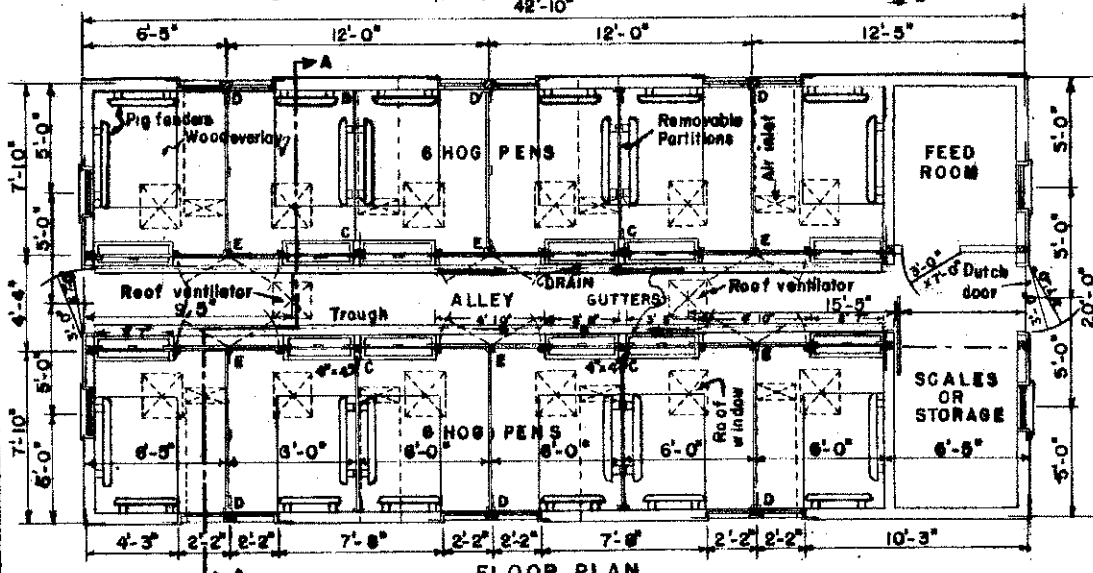
FLOOR PLAN Scale 1/4" = 1'-0"
