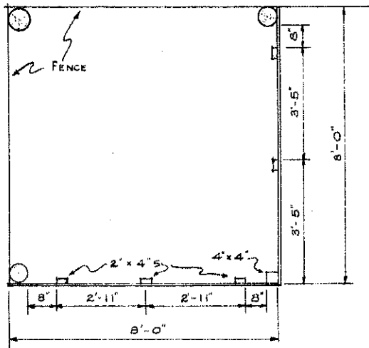
PLAN SCALE \frac{1}{2}'' = 1'-0''
