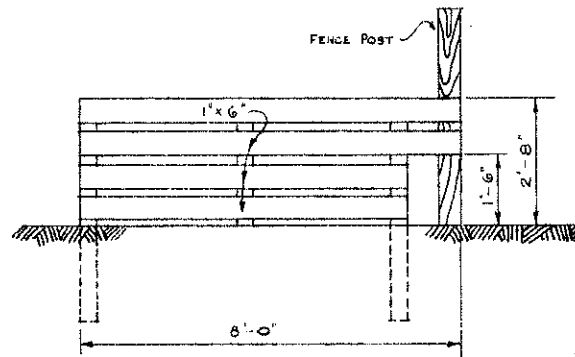
SOUTH ELEVATION SCALE \frac{1}{2}'' = 1'-0''
