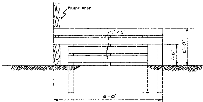
WEST ELEVATION SCALE \frac{1}{2}'' = 1'-0''
