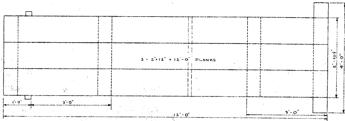
PLAN OF FLOOR SCALE 1"=1'-0"
