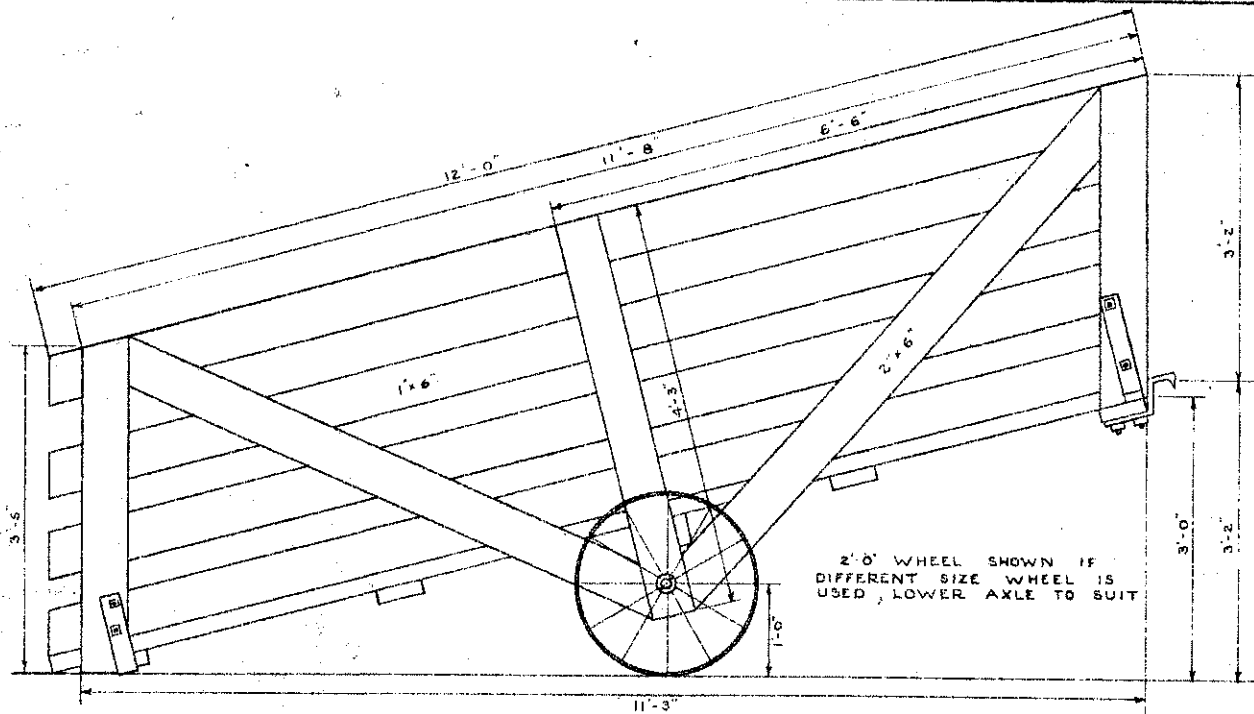
SIDE ELEVATION SCALE 1"=1'-0"
