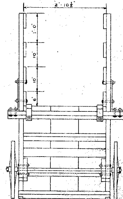
FRONT END ELEVATION SCALE 1"=1'-0"
