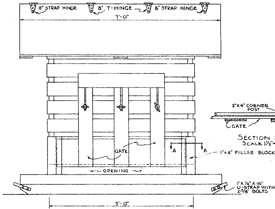
SIDE VIEW SCALE 1"=1'-0"
