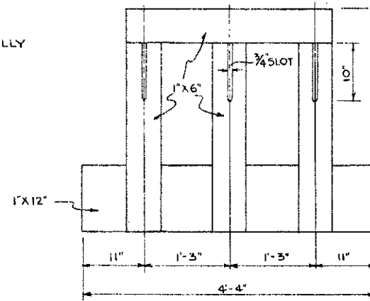
DETAIL OF GATE SCALE 1"=1'-0"
