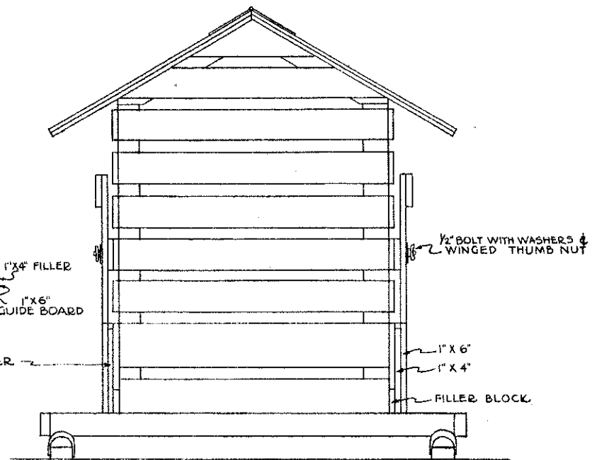
END VIEW SCALE 1"=1'-0"
