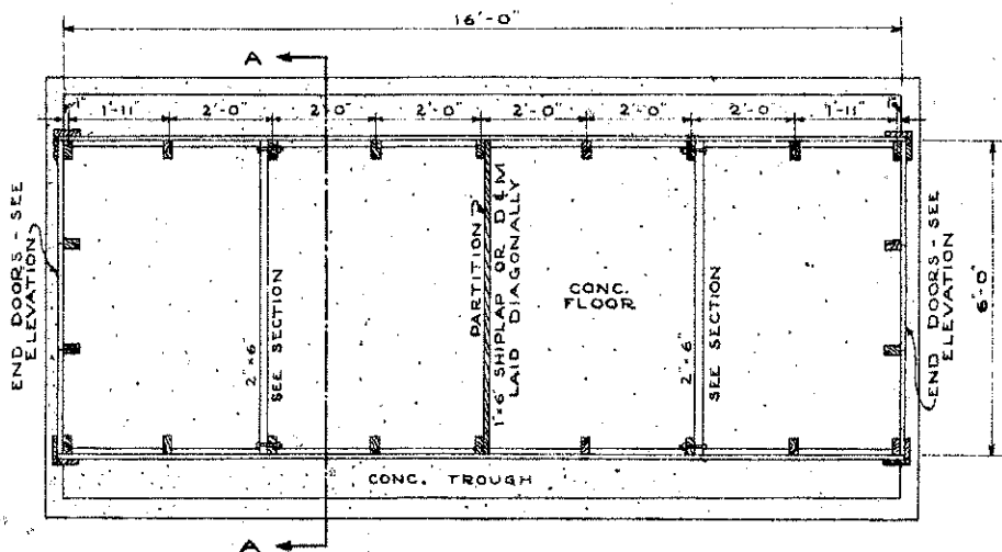
PLAN SCALE 1/2" = 1'-0"
