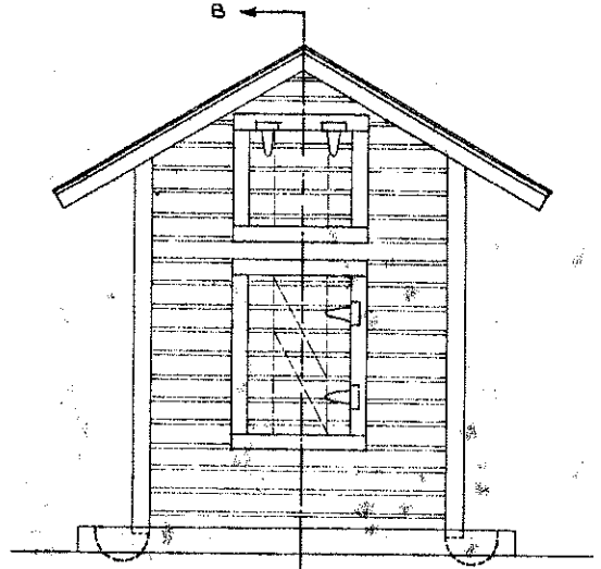
END ELEVATION SCALE 1/2" = 1'-0"
