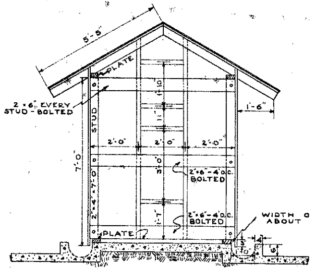
SECTION A-A SCALE 1/2" = 1'-0"
