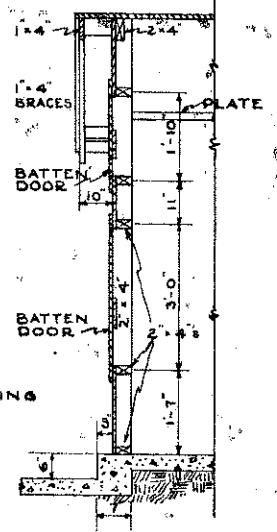
SECTION B-B SCALE 1/2" = 1'-0"
