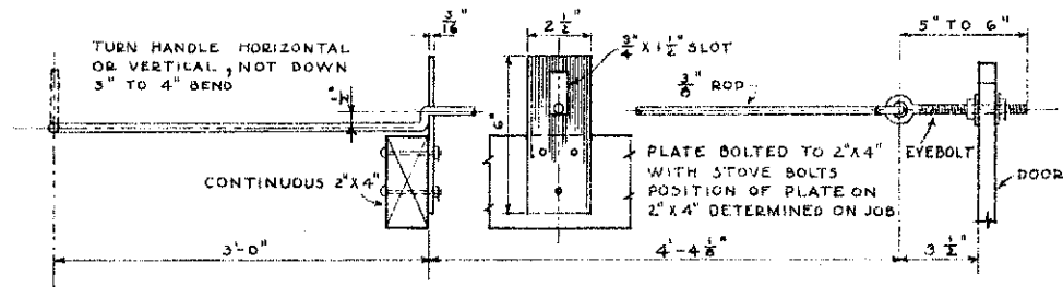
DOOR OPERATING LEVER SCALE 3" = 1'-0"
