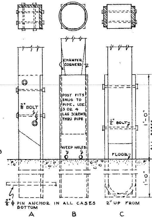
FLOOR ANCHORS FOR 4"x4" WOOD POSTS SCALE 3" = 1'-0"
