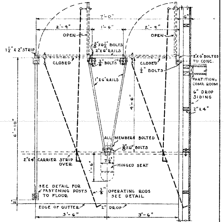
PLAN OF TWO STALLS SCALE 3/4" = 1'-0"
