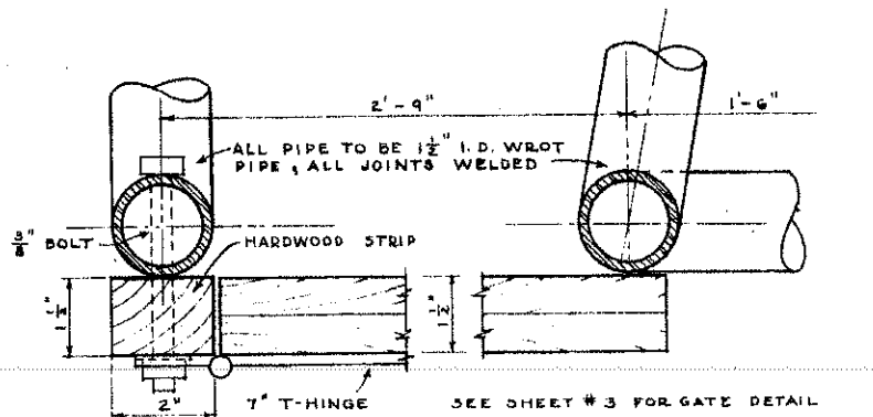
METHOD OF SWINGING GATES TO PIPE PARTITIONS SCALE 1/2" = 1'-0"
