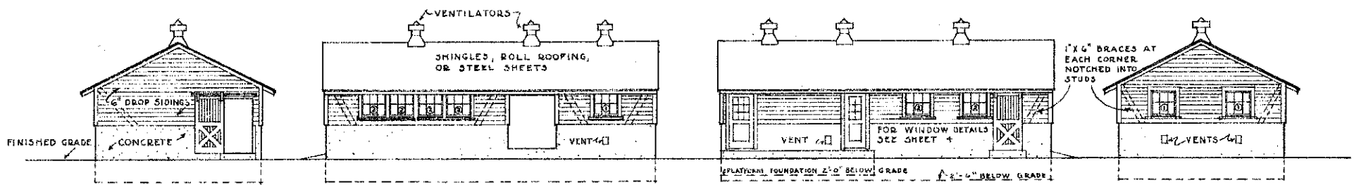
ELEVATIONS SCALE \frac{1}{8}'' = 1'-0''
