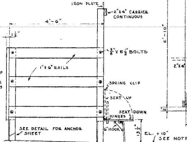
ELEVATION, CENTER PARTITIONS
