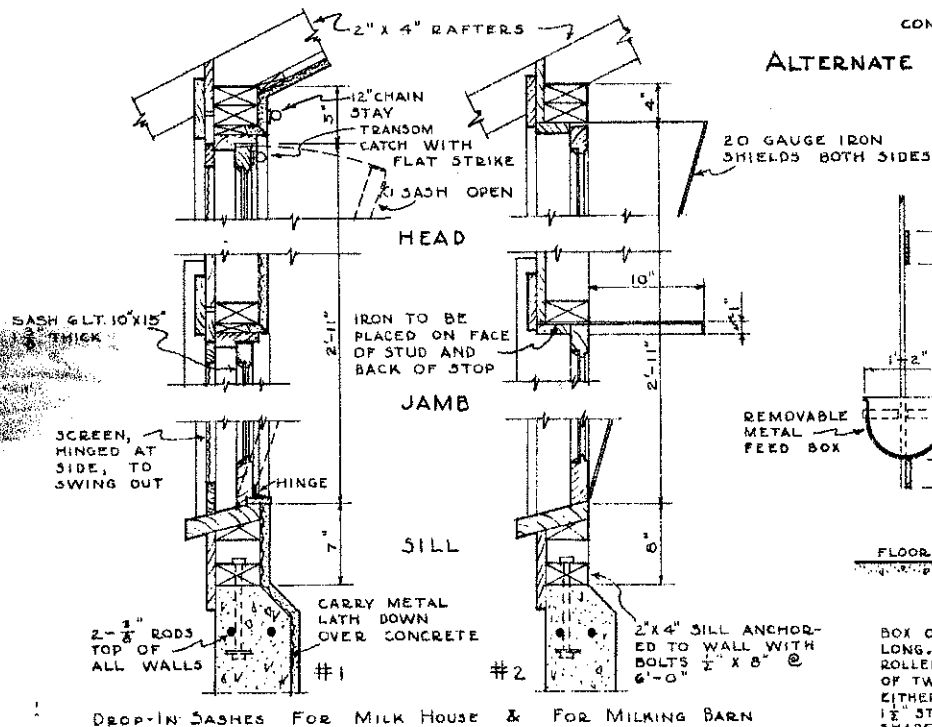
TYPICAL WINDOW DETAILS SCALE 1 1/2" = 1'-0"
