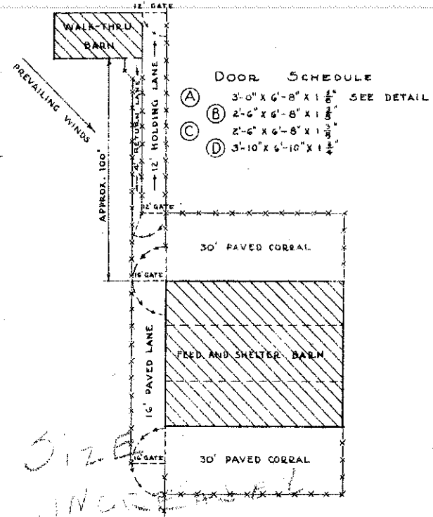
PLOT PLAN SCALE 1" = 30'
