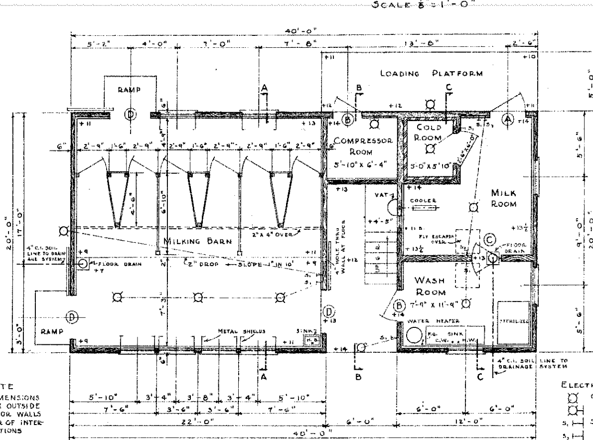
FLOOR PLAN SCALE \frac{1}{4}'' = 1'-0''
