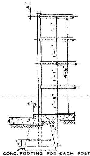
ALTERNATE DETAIL - PIPE PARTITIONS SCALE 3/4" = 1'-0"
