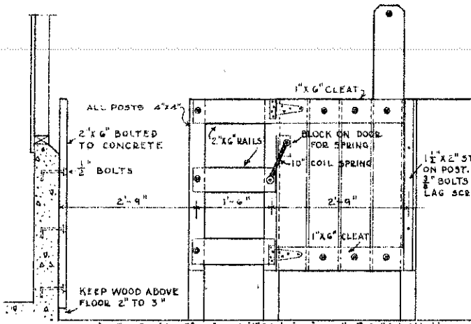
ELEVATION OF GATES FROM EXIT ALLEY
