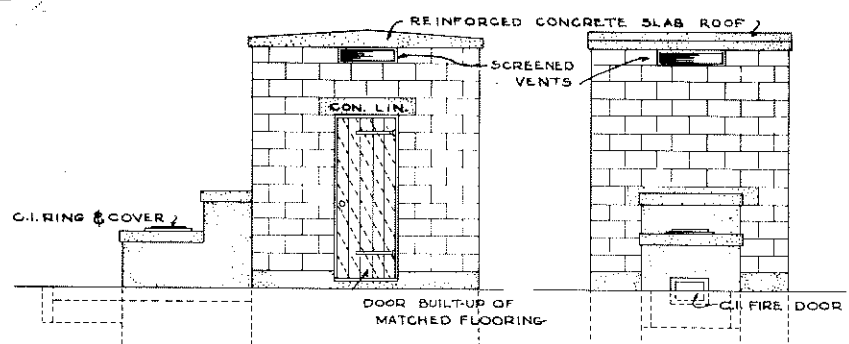
FRONT ELEVATION SCALE \frac{1}{4}'' = 1'-0'' SIDE ELEVATION SCALE \frac{1}{4}'' = 1'-0''
