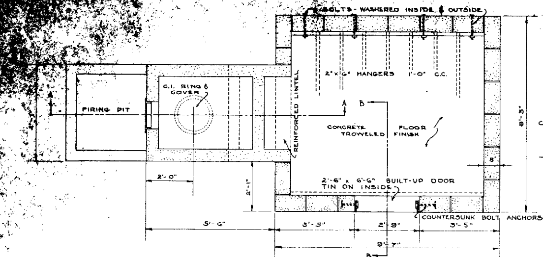
PLAN SCALE \frac{1}{2}'' = 1'-0''
