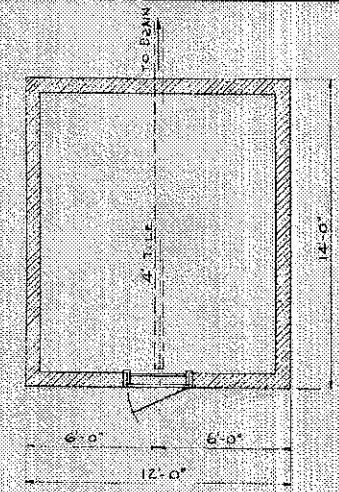
PLAN SCALE 1/4" = 1'-0"
