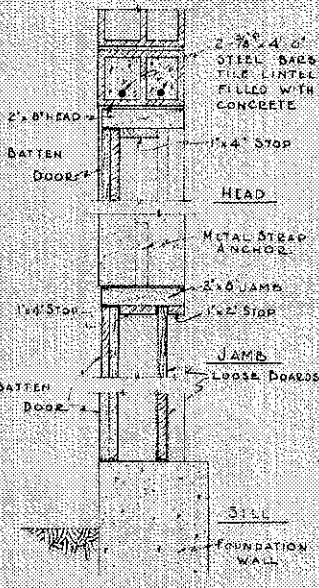
DETAILS OF DOOR SCALE 1/8" = 1'-0"
