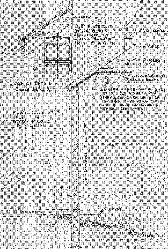
SECTION TIED CLAY TILE OR CONCRETE BLOCK WALL SCALE 1/8" = 1'-0"
