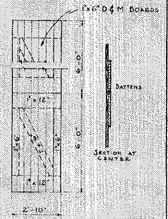
ELEV. OF DOOR DIMENSIONS GIVEN ARE ONLY APPROXIMATE. EXACT DIMENSIONS DEPEND ON BLOCKS USED.
