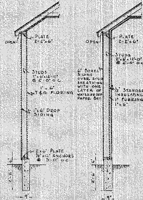
ALTERNATE WALL SECTIONS USING FRAME CONSTRUCTION SCALE 1/8" = 1'-0"
