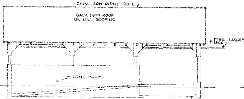
SIDE ELEVATION SCALE OF ELEVATIONS 1/16" = 1'-0"
