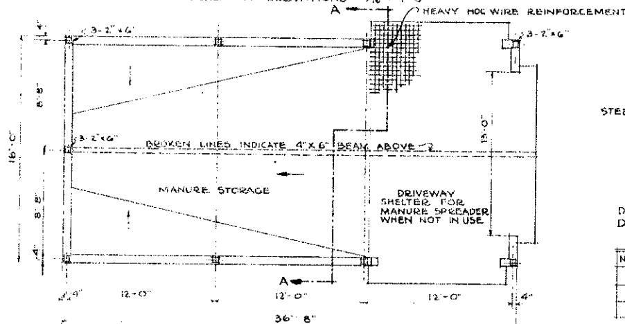
PLAN SCALE 1/16" = 1'-0"
