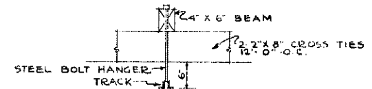
DETAIL SHOWING TRACK AND SUPPORTS SCALE 1/4" = 1'-0"
