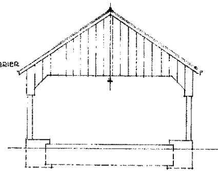
END ELEVATION - DRIVEWAY END
