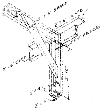
ISOMETRIC VIEW OF POST CONSTRUCTION
