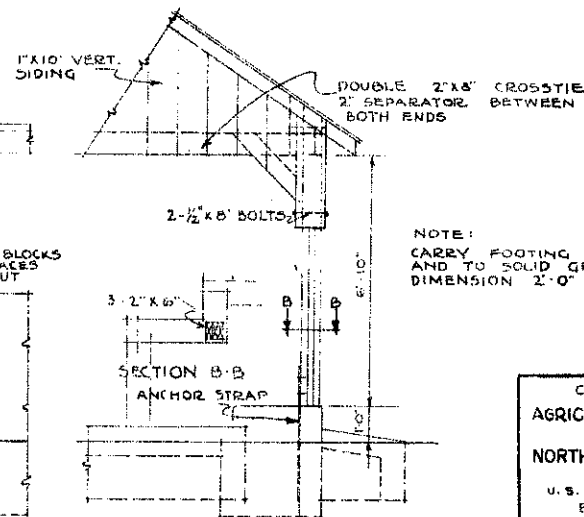
CORNER POST DETAIL OF BRACING SCALE 3/8" = 1'-0"
