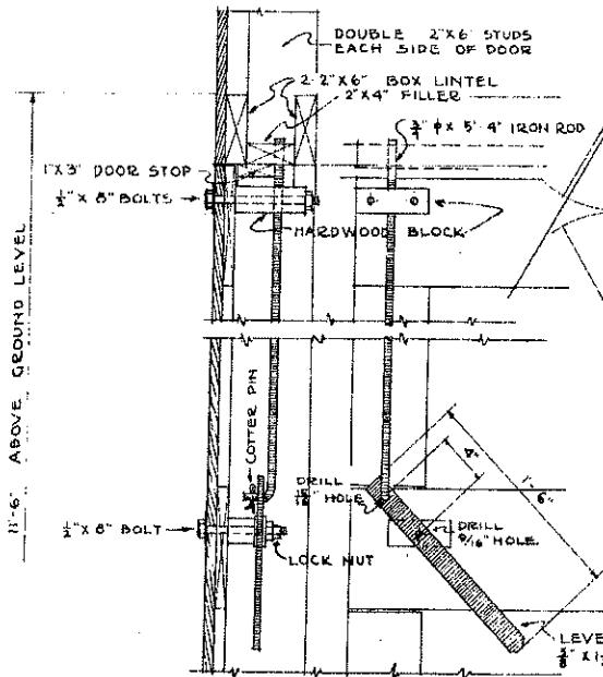
SECTION INSIDE ELEVATION DETAIL OF LOCKING DEVICE FOR SWINGING DOOR SCALE 1\frac{1}{2}" = 1'-0"
