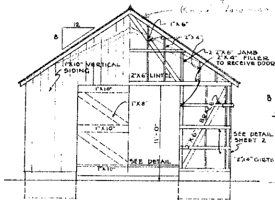
END ELEVATION SCALE \frac{1}{8}" = 1'-0"
