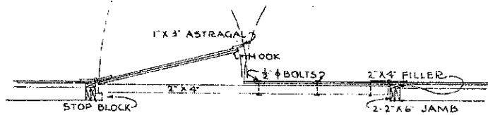
BAR FOR BOTTOM OF HINGED DOORS SCALE \frac{3}{8}" = 1'-0"
