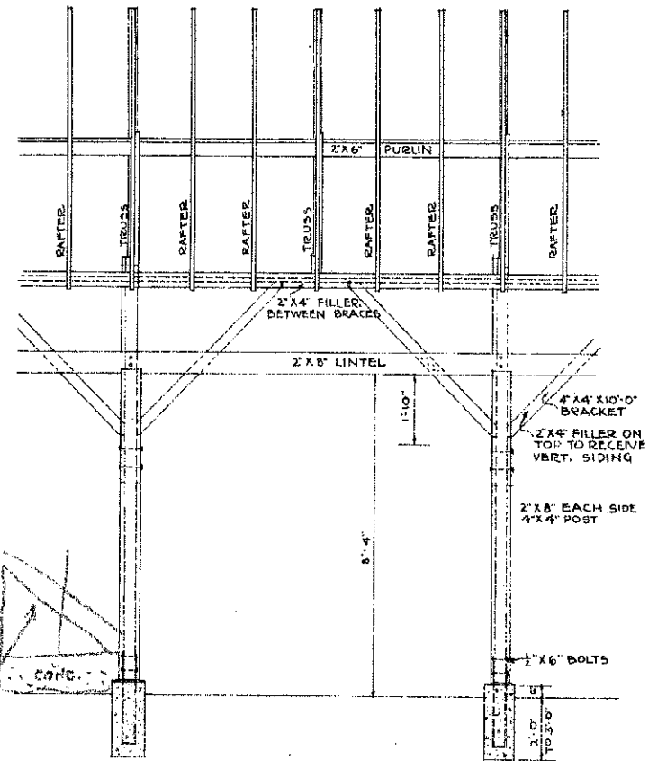
DETAIL OF BRACING SCALE 3/8" = 1'-0"
