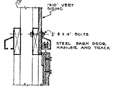
DETAIL OF LINTEL OVER ROLLING DOORS
