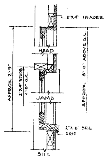
CROSS SECTION SCALE 3/8" = 1'-0"
