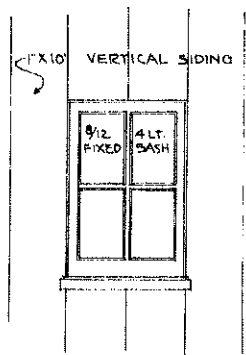
ELEVATION SCALE 1/2" = 1'-0"
