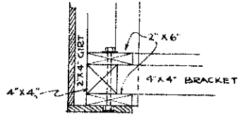
DETAIL CORNER POST (SECT B-D) SCALE 1\frac{1}{2}" = 1'-0"
