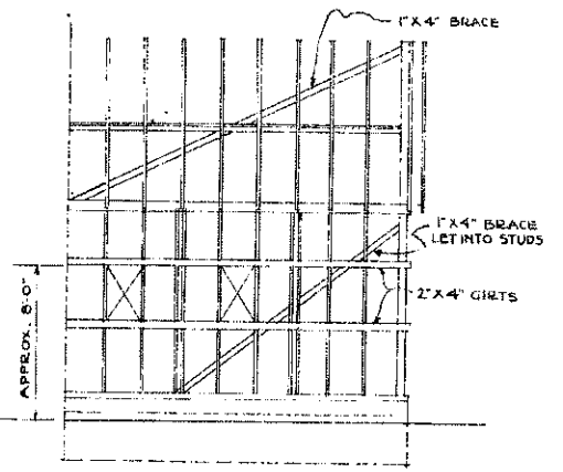
FRAMING DIAGRAM OF REAR WALL SCALE \frac{1}{4}" = 1'-0"
