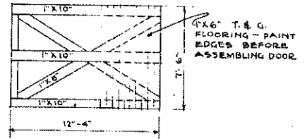
SLIDING DOOR SCALE \frac{3}{16}" = 1'-0"
