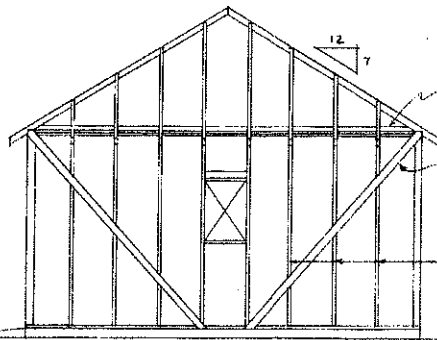
SIDE ELEVATION
