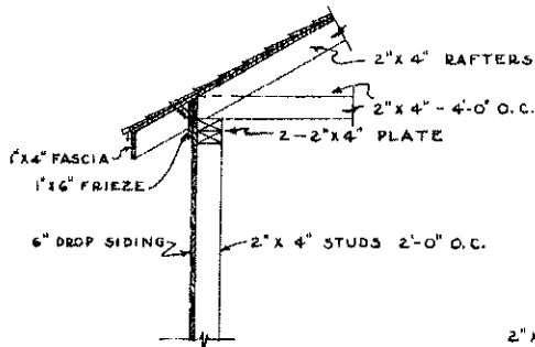
DETAIL OF CORNICE SCALE \frac{3}{4}'' = 1'-0''
