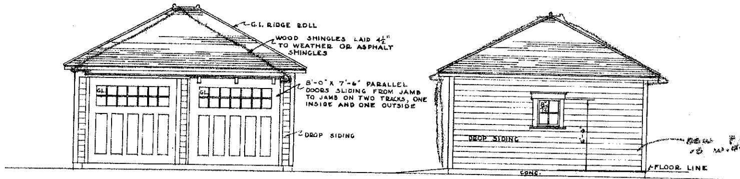
FRONT ELEVATION SCALE \frac{1}{4}'' = 1'-0''
