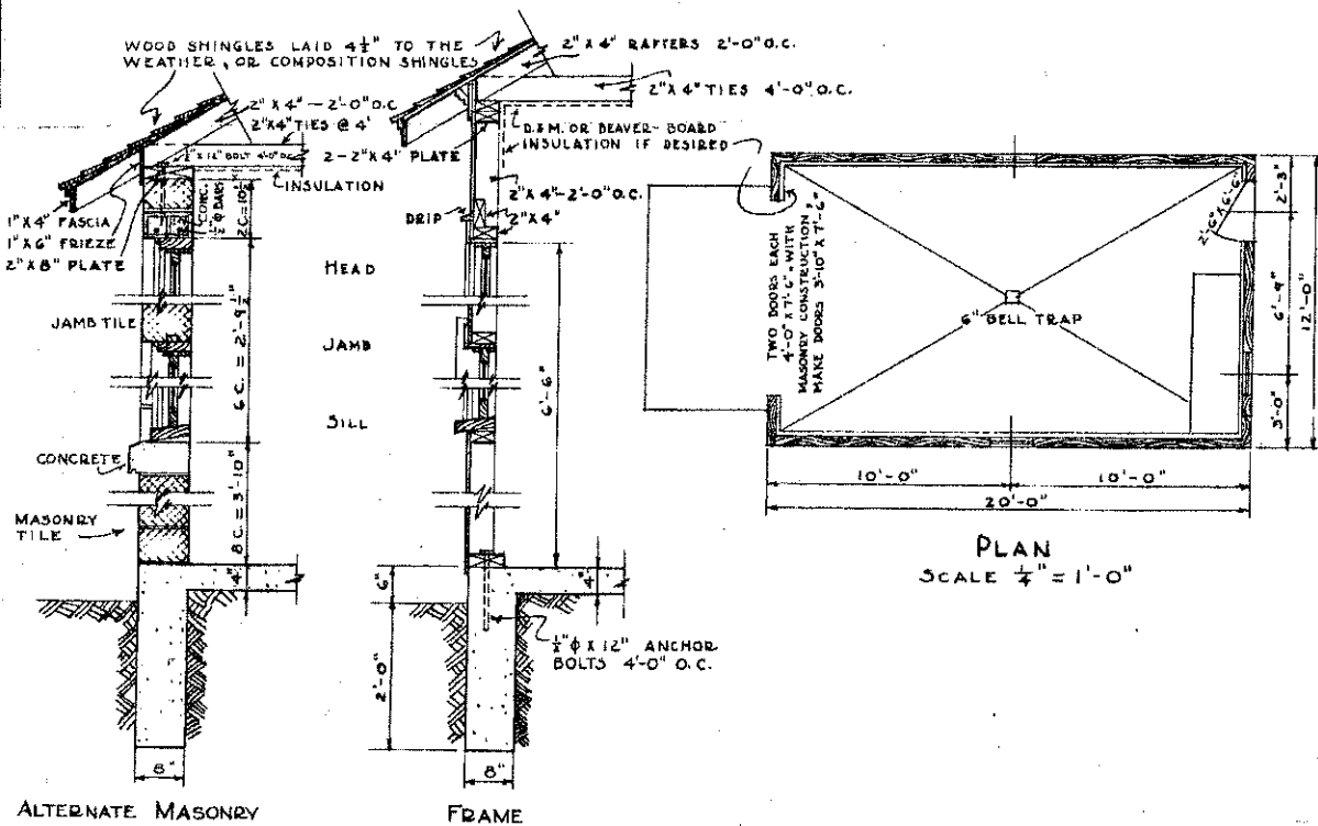
WALL CONSTRUCTIONS SCALE \frac{3}{8}'' = 1'-0''
