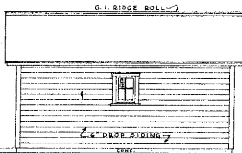
SIDE ELEVATION SCALE \frac{1}{4}'' = 1'-0''
