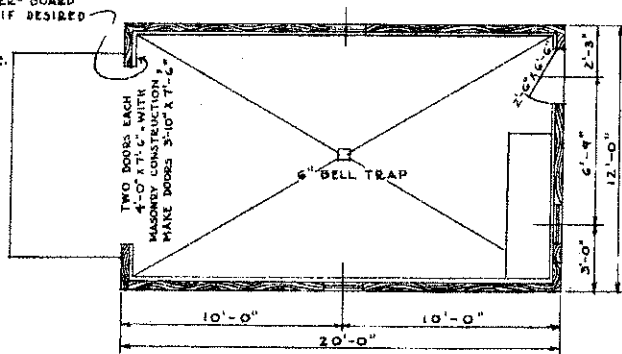
PLAN SCALE \frac{1}{4}'' = 1'-0''
