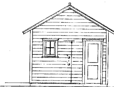
REAR ELEVATION SCALE \frac{1}{4}'' = 1'-0''
