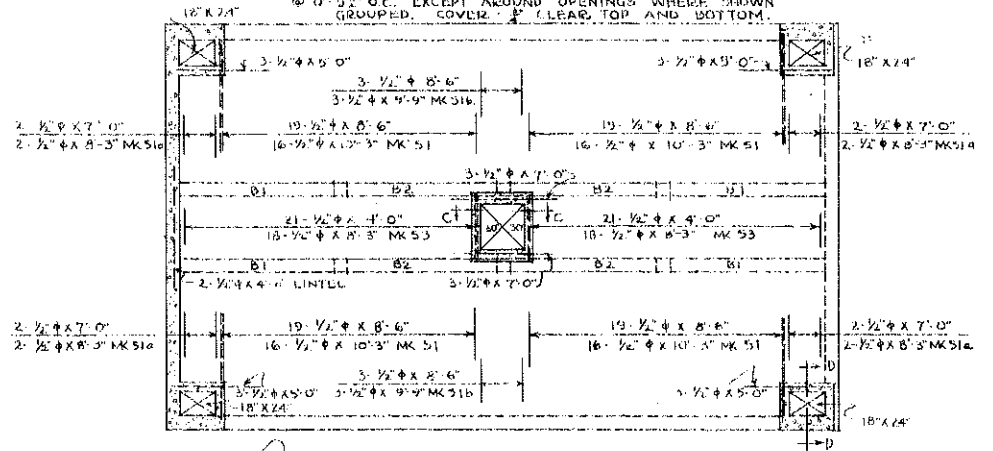
ROOF PLAN SHOWING PLACEMENT OF STEEL SCALE 3/16" = 1'-0"
