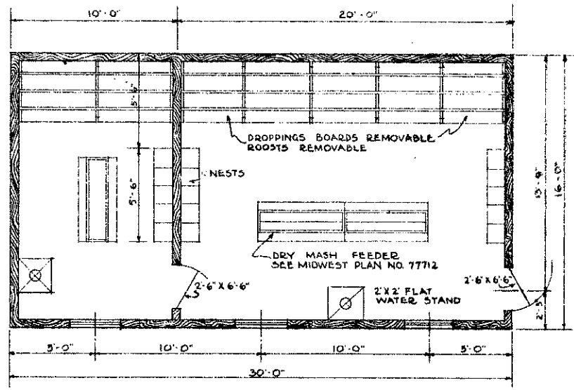
PLAN SCALE \frac{1}{4} " = 1'-0"
