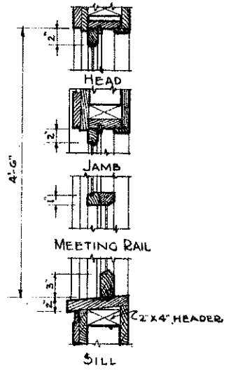
WINDOW DETAILS SCALE \frac{1}{2} " = 1'-0"
