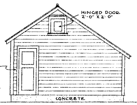
END ELEVATION SCALE \frac{1}{4} " = 1'-0"
