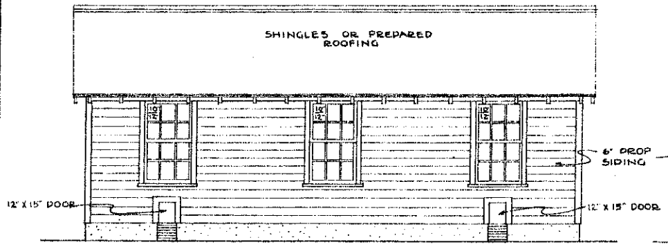
FRONT ELEVATION SCALE \frac{1}{4} " = 1'-0"
