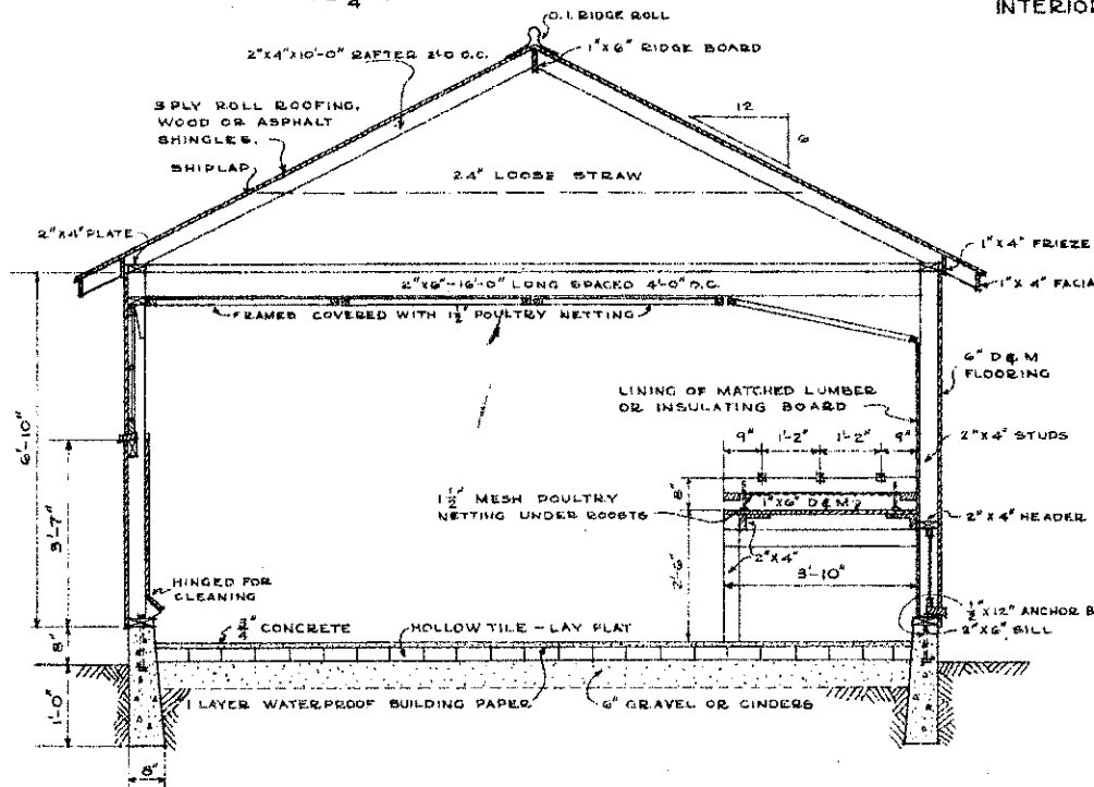
SECTION SCALE \frac{1}{2}'' = 1'-0''
