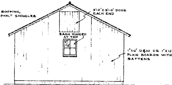
EAST ELEVATION (WEST SIMILAR) SCALE \frac{1}{4}'' = 1'-0''
