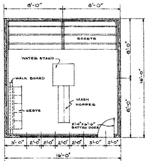
FLOOR PLAN SCALE \frac{1}{4}'' = 1'-0''
