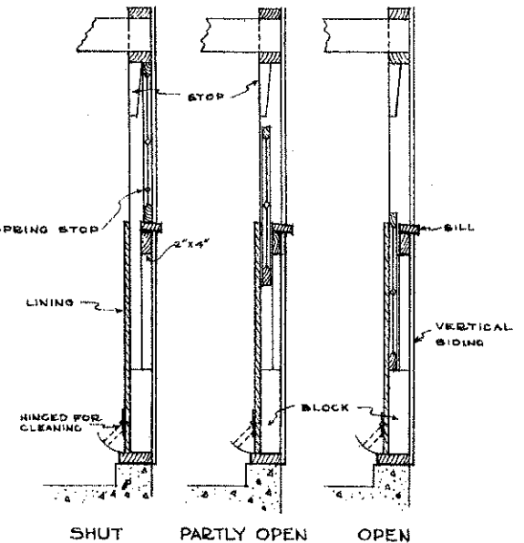
WINDOW DETAILS SCALE \frac{3}{4}'' = 1'-0''
