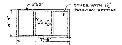
PLAN OF STRAW FRAMES (8 REQUIRED) SCALE \frac{1}{4}'' = 1'-0''
