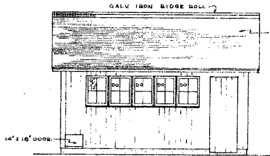
SOUTH ELEVATION SCALE \frac{1}{4}'' = 1'-0''
