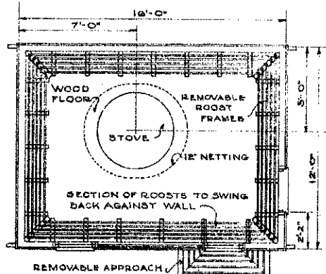
FLOOR PLAN SCALE \frac{1}{4} " = 1'-0"
