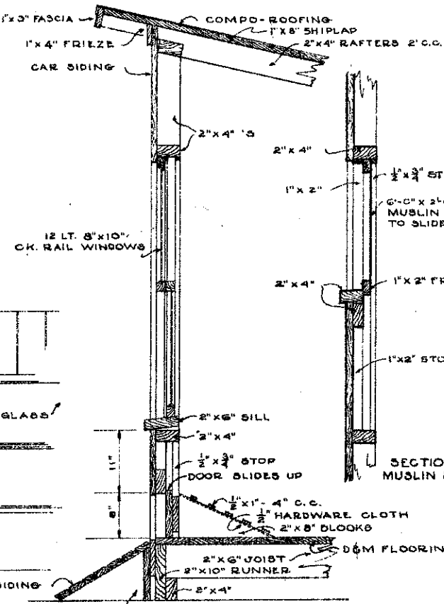
SECTION OF FRONT WALL WALL DETAILS SCALE 1" = 1'-0"
