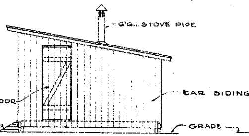
RIGHT ELEVATION SCALE \frac{1}{4} " = 1'-0"
