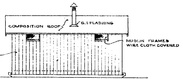
REAR ELEVATION SCALE \frac{1}{4} " = 1'-0"
