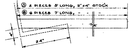
FRAMING DETAILS
