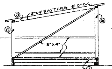
WEST END FRAMING SCALE 3/4" = 1'-0"
