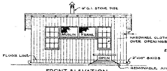
FRONT ELEVATION SCALE \frac{1}{4} " = 1'-0"
