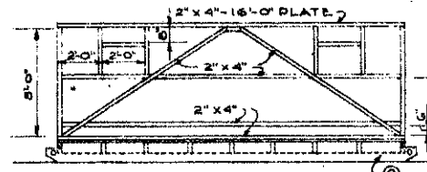
REAR WALL FRAMING SCALE 3/4" = 1'-0"
