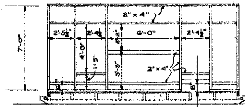
FRONT WALL FRAMING SCALE 3/4" = 1'-0"
