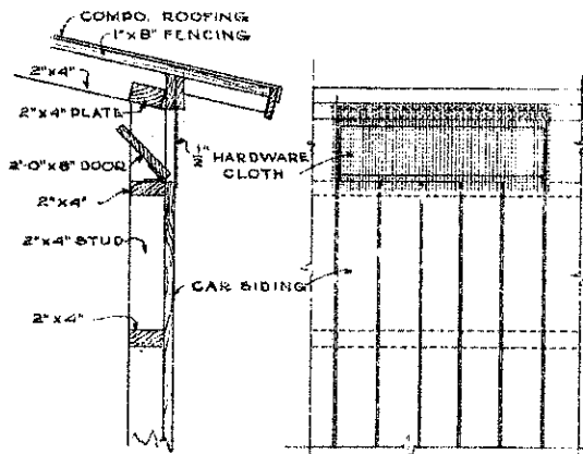
SECTION THRU VENTILATOR SCALE 1" = 1'-0"
