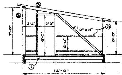
EAST END FRAMING SCALE 3/4" = 1'-0"
