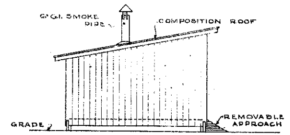
LEFT ELEVATION SCALE \frac{1}{4} " = 1'-0"
