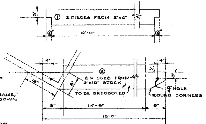
REAR WALL FRAMING SCALE 3/4" = 1'-0"
