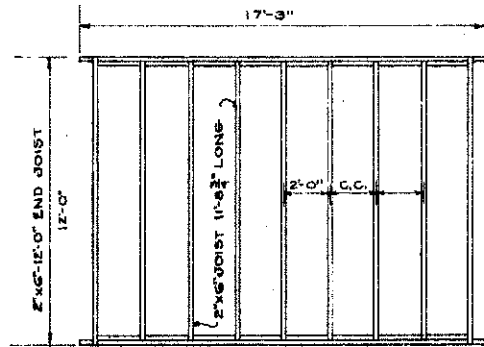
FLOOR FRAMING SCALE 3/4" = 1'-0"
