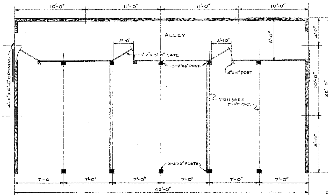
FLOOR PLAN SCALE \frac{1}{4}'' = 1'-0''
