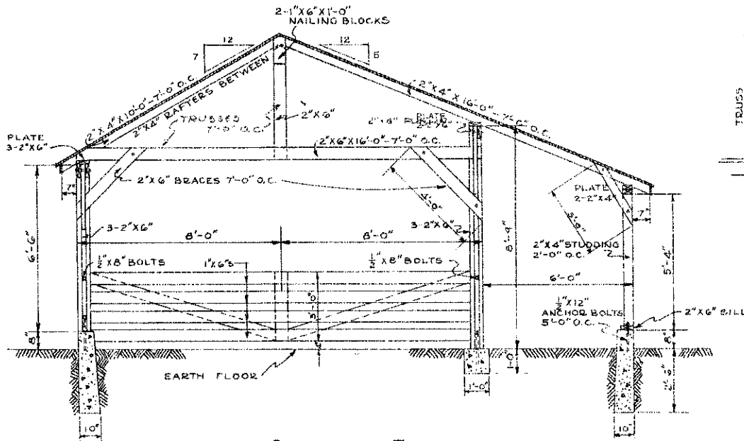
DETAIL OF TRUSS SCALE \frac{3}{8}'' = 1'-0''
