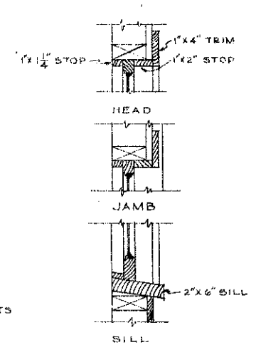
WINDOW DETAILS SCALE 1\frac{1}{2}'' = 1'-0''
