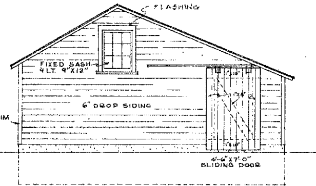
END ELEVATION SCALE \frac{1}{4}'' = 1'-0''
