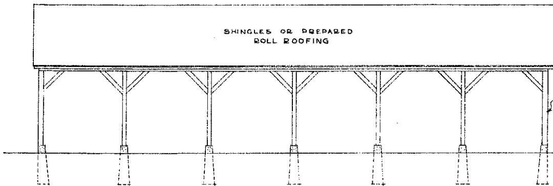
FRONT ELEVATION SCALE \frac{1}{4}'' = 1'-0''
