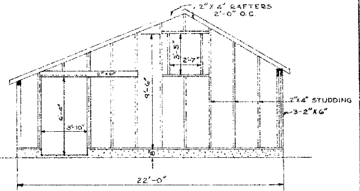
END FRAMING PLAN SCALE \frac{1}{4}'' = 1'-0''
