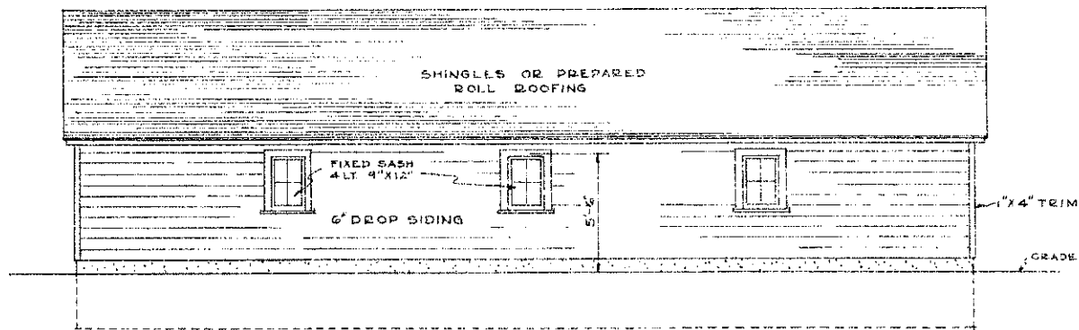
REAR ELEVATION SCALE \frac{1}{4}'' = 1'-0''
