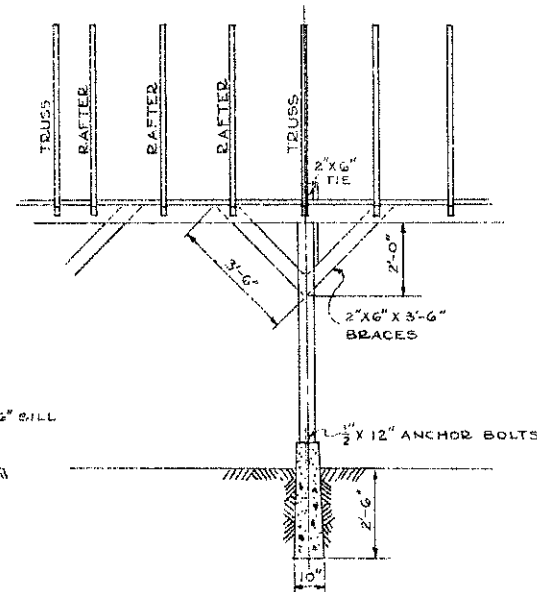
DETAIL OF BRACING SCALE \frac{3}{8}'' = 1'-0''
