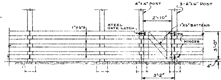
DETAIL OF ALLEY PARTITION AND GATE SCALE \frac{3}{8}'' = 1'-0''
