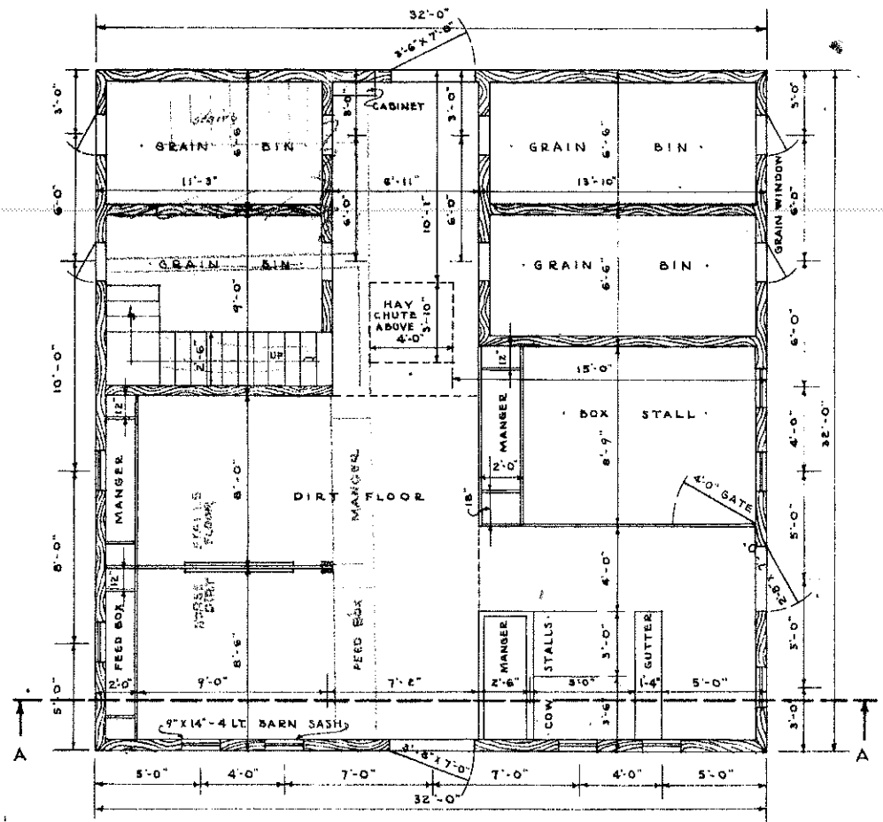
FLOOR PLAN SCALE \frac{1}{4}" = 1'-0"
