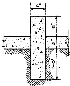
SECTION X-X SCALE 1" = 1'-0"
