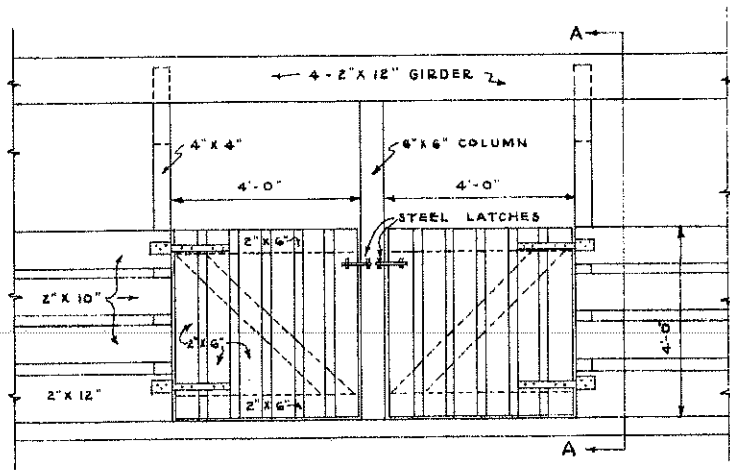
DETAIL OF BOX STALL FRONT SCALE \frac{1}{2} " = 1'-0"
