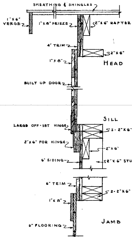
LARGE HAY DOOR DETAILS SCALE \frac{1}{2} " = 1'-0"
