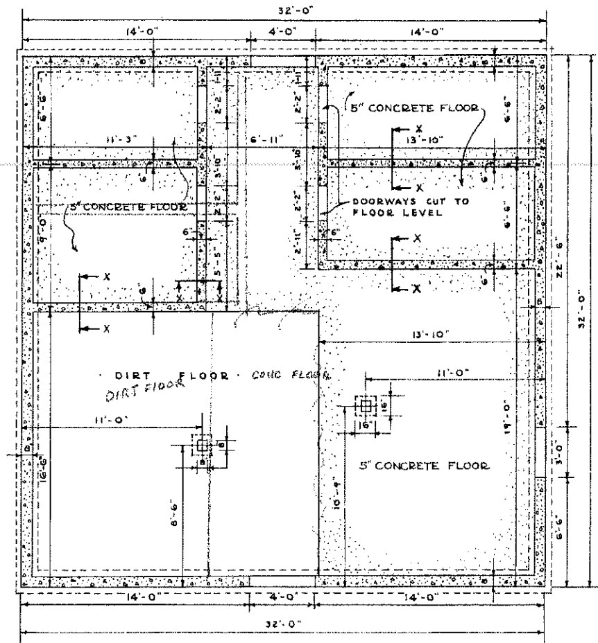
FOUNDATION PLAN SCALE \frac{1}{4}" = 1'-0"
