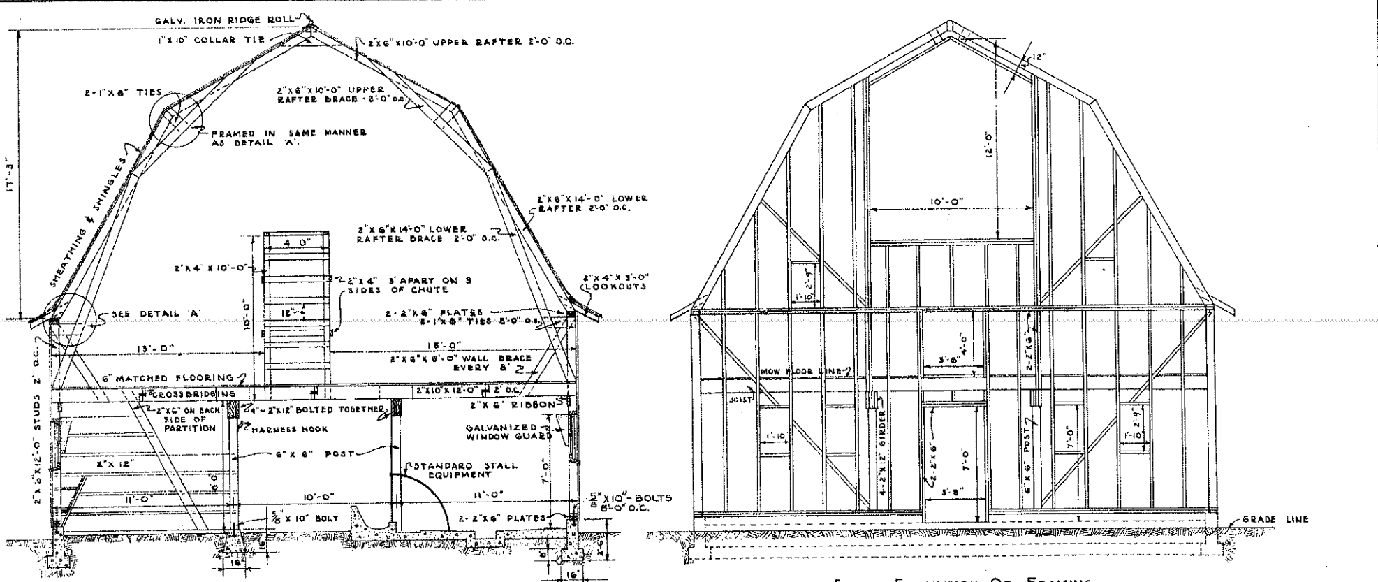
CROSS SECTION A-A SCALE \frac{1}{4}'' = 1'-0''
