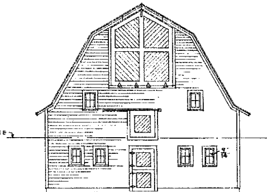
SOUTH ELEVATION SCALE \frac{1}{8}'' = 1'-0''
