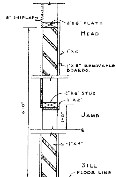
DETAIL OF GRAIN DOOR SCALE 1" = 1'-0"
