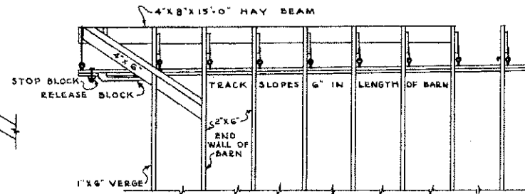
ELEVATION OF HOOD FRAMING SCALE \frac{1}{8} " = 1'-0"
