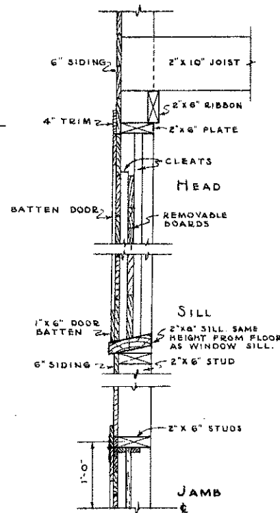
DETAIL OF GRAIN WINDOW SCALE 1" = 1'-0"
