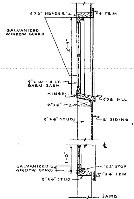
WINDOW DETAILS SCALE 1'' = 1'-0''
