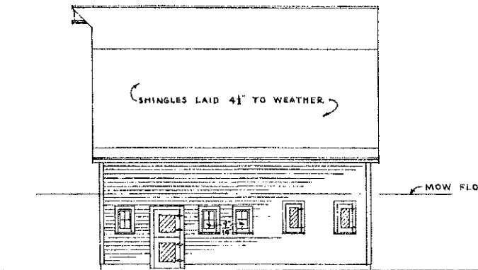
EAST ELEVATION SCALE \frac{1}{8}'' = 1'-0''
