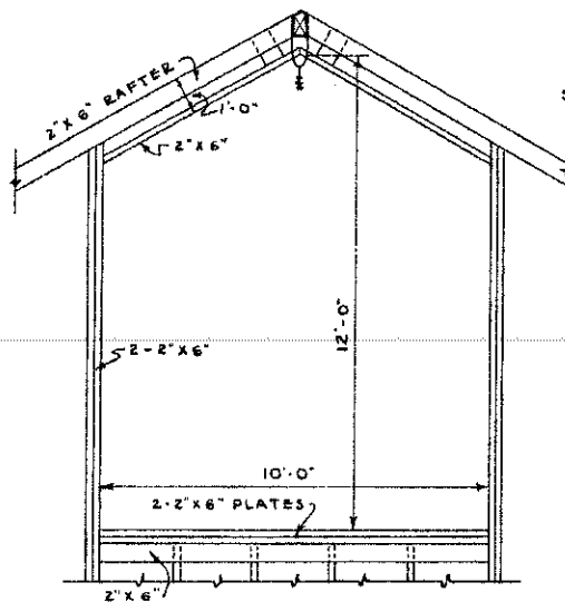
LARGE HAY DOOR FRAMING SCALE \frac{1}{8} " = 1'-0"
