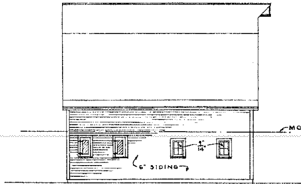
WEST ELEVATION SCALE \frac{1}{8}'' = 1'-0''
