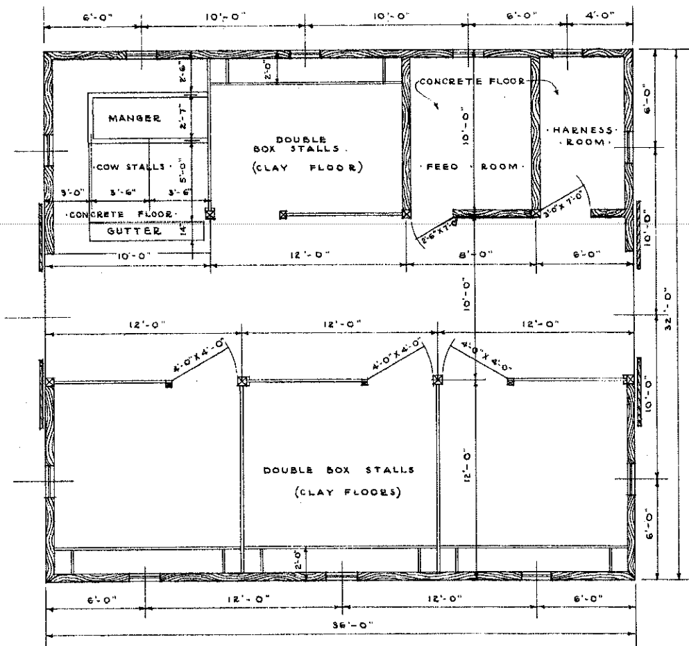
ALTERNATE FLOOR PLAN SCALE \frac{1}{4} " = 1'-0"
