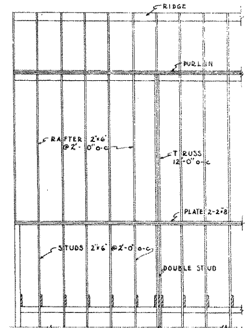
PART SIDE ELEVATION OF ROOF FRAMING SCALE 1/4" = 1'-0"
