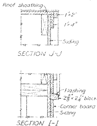
SECTION I-I
