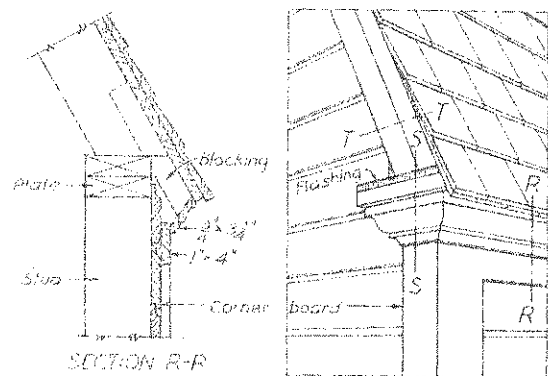
CORNICE NO-2
