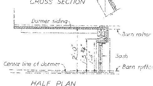
DORMER DETAILS
