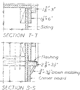
SECTION S-S
