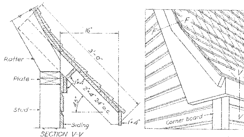
CORNICE NO-4
