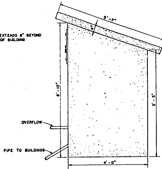
SIDE ELEVATION
