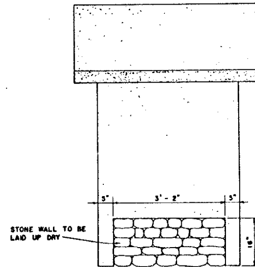
REAR ELEVATION
