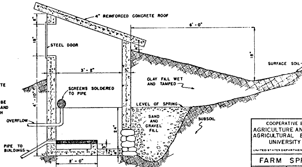
CROSS SECTION ON LINE A-A
