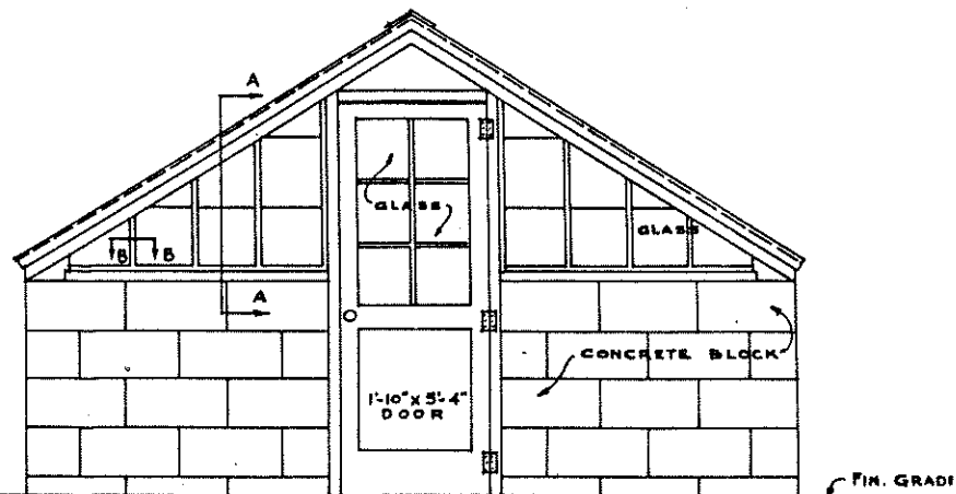
END ELEVATION SCALE \frac{1}{4} " = 1'-0"
