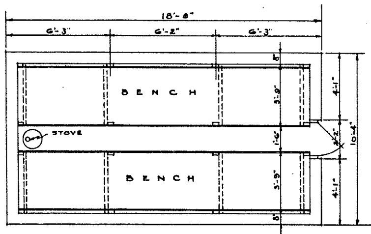
PLAN SHOWING ARRANGEMENT OF BENCHES SCALE \frac{1}{8} " = 1'-0"
