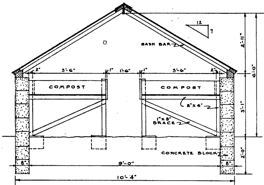
END SECTION SCALE \frac{1}{4} " = 1'-0"
