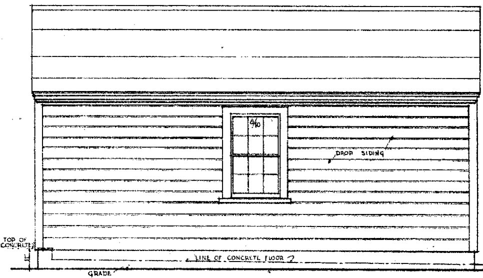
LEFT SIDE ELEVATION (RIGHT SIDE SIMILAR)
