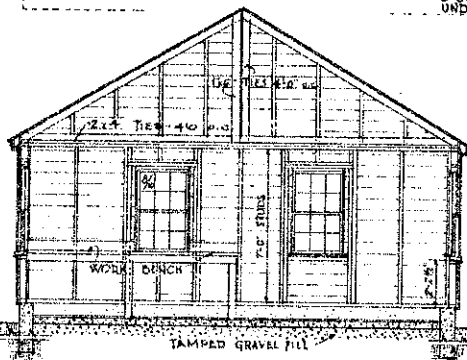
TRANSVERSE SECTION
