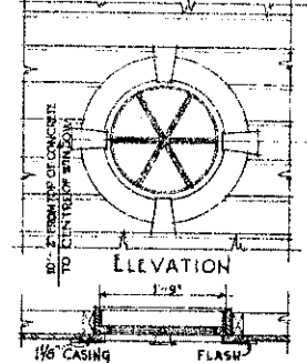
SECTION DETAIL OF ROUND WINDOW
