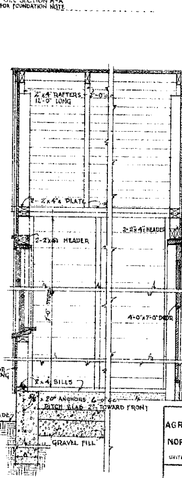
SECTION B-B
