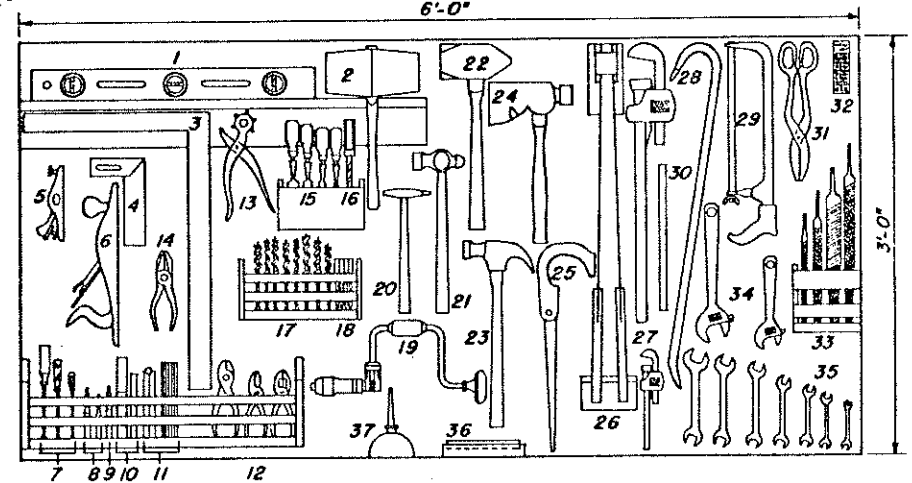
TOOL PANEL
