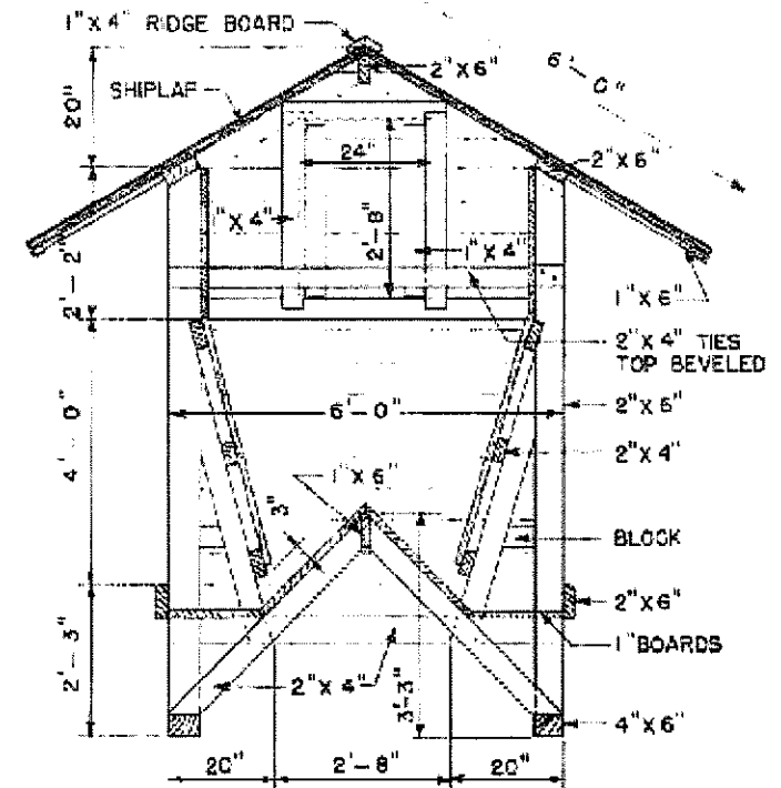
CROSS SECTION
