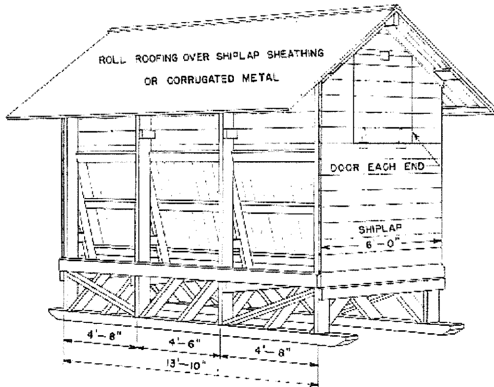
PERSPECTIVE
