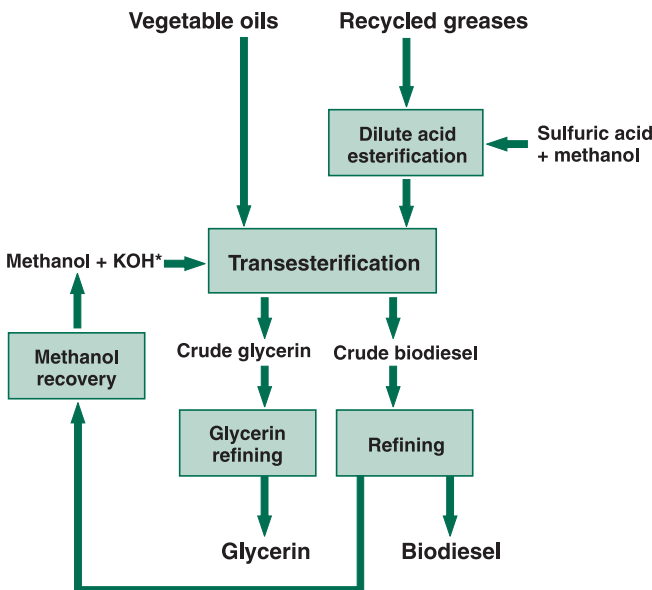
Figure 1. Basic Process Technology.
