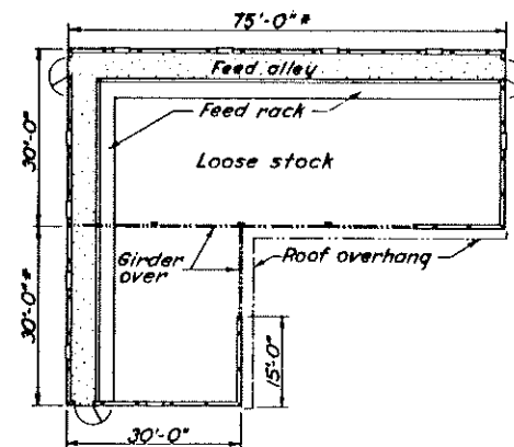
PLAN WITH ELL
